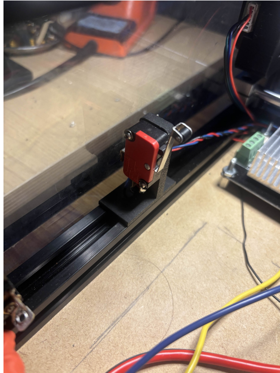
Figure 49: Limit bumper mounted to the aluminum frame.
