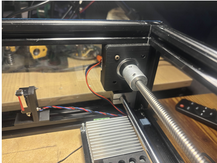
Figure 48: Stepper motor mount bracket.
