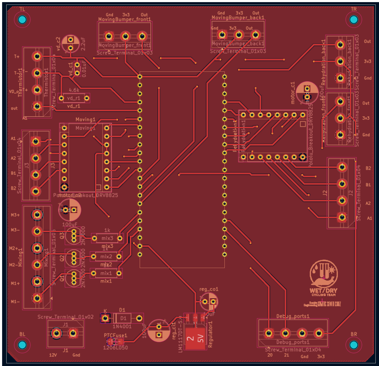
Figure 37: Top layer of designed PCB
