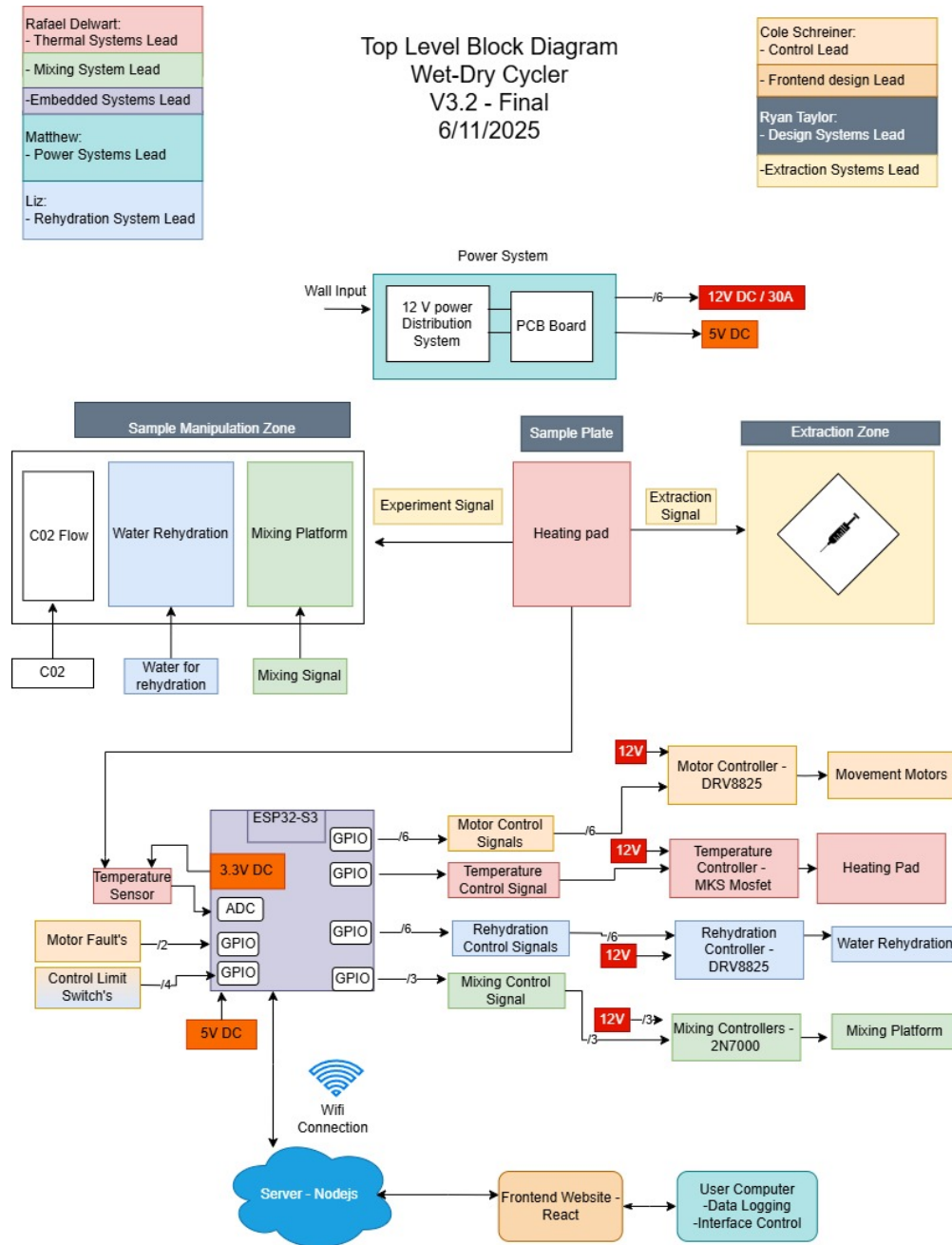
Figure 1: Overall system block diagram
