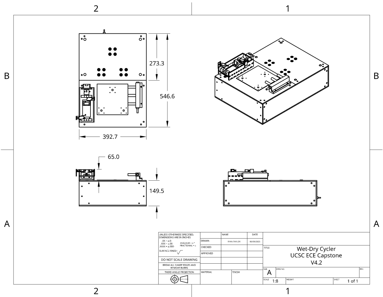
Figure 42: Dimensioned drawing of wet/dry Cyclor housing with annotated panel and frame sizes (mm).
