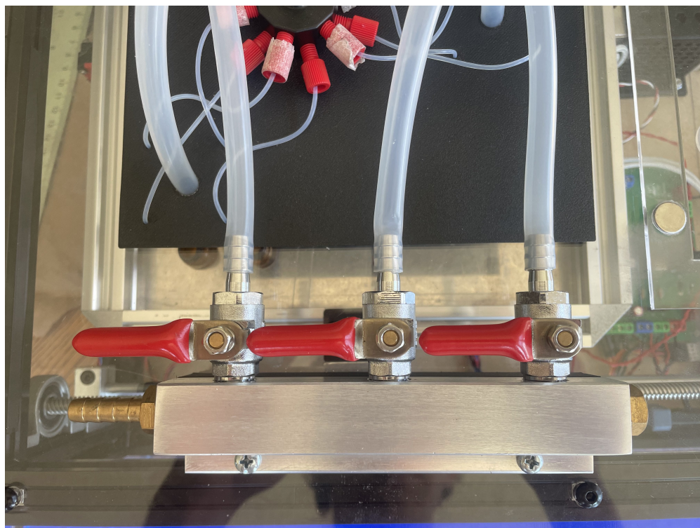
Figure 7: CO 2 manifold mounted on top of the device, controlling three output zones.
