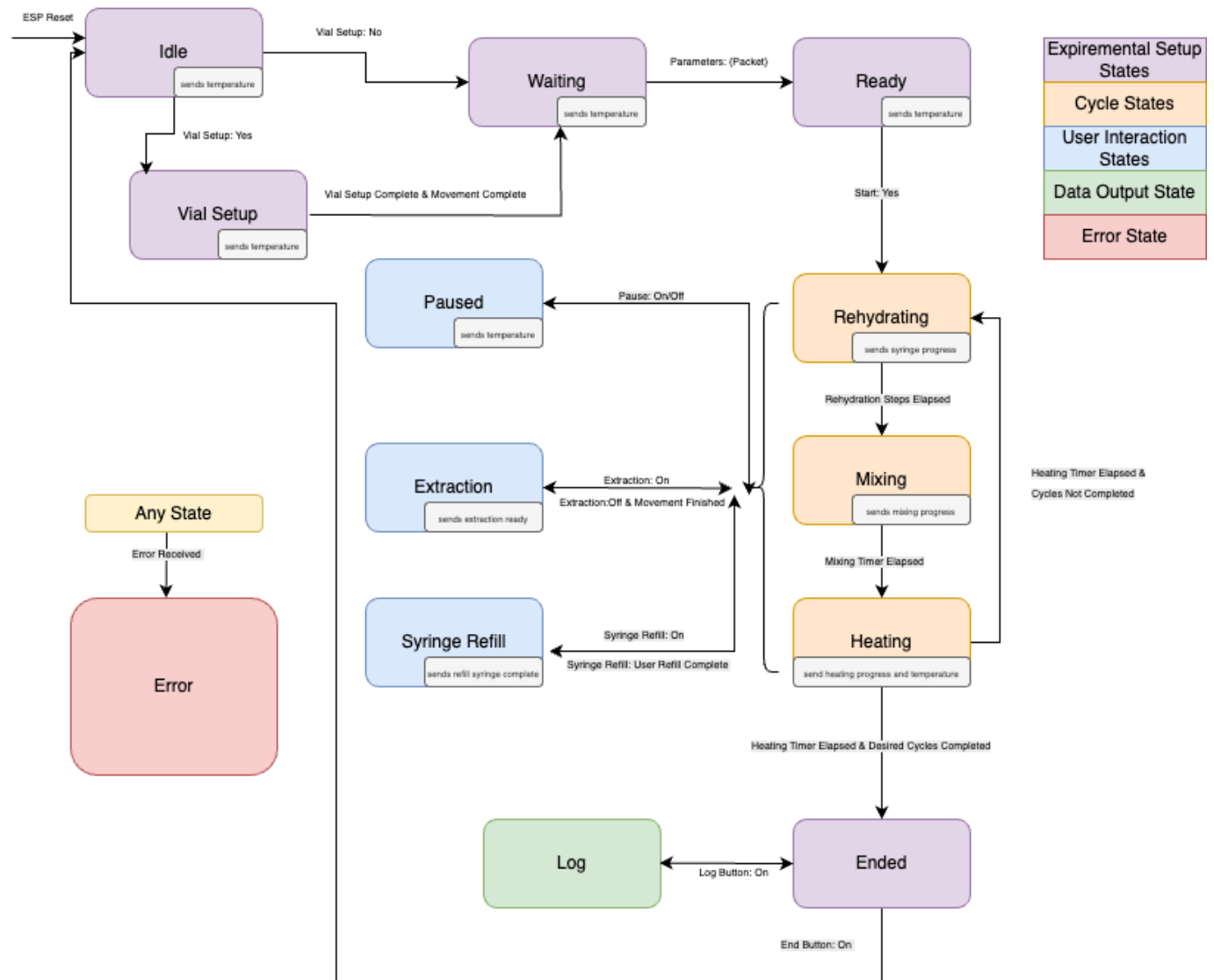
Figure 30: State machine diagram for the embedded control system. Arrows indicate valid transitions based on input events and subsystem completion.
