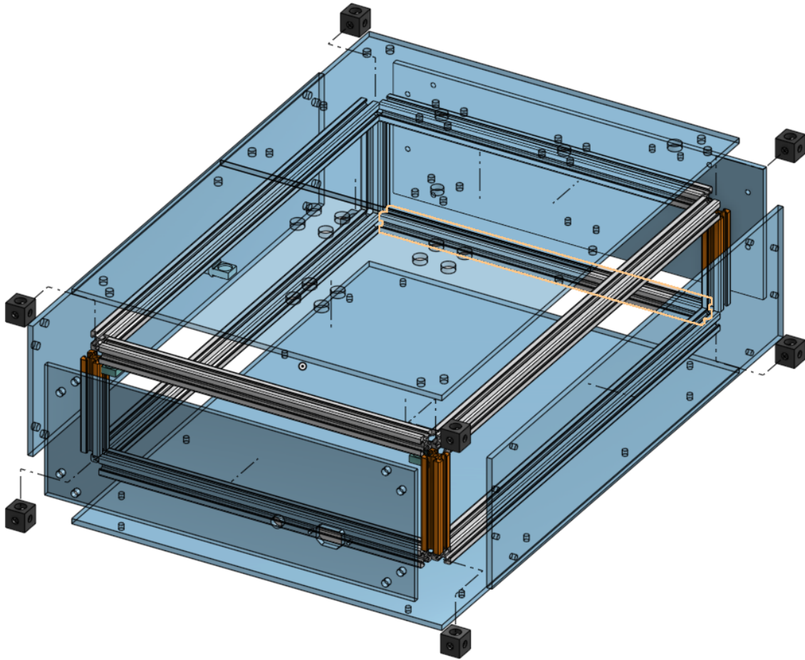
Figure 45: Exploded CAD view showing panel-frame interface and bracket positions.
