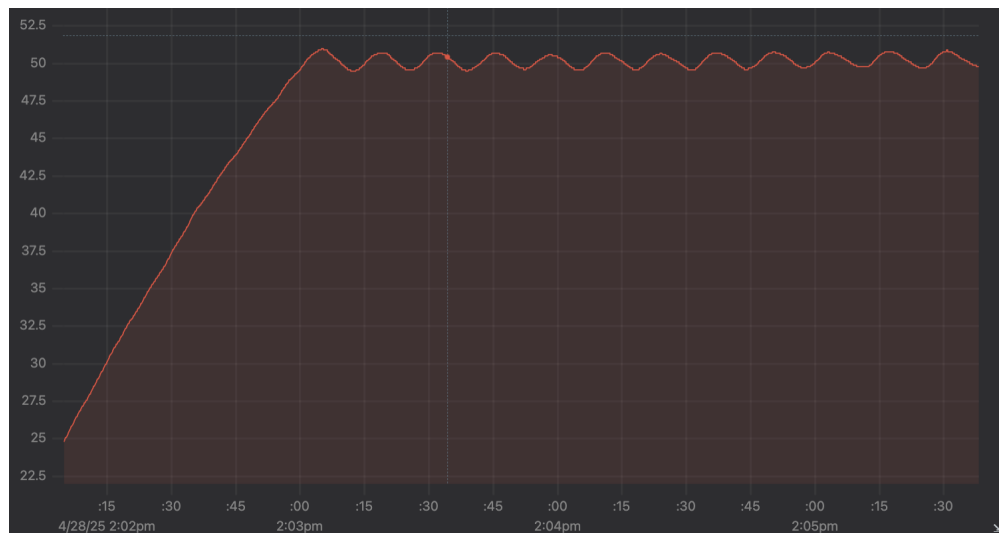
Figure 5: Temperature profile over five minutes, showing the heating pad warming from ambient to 50°C.
