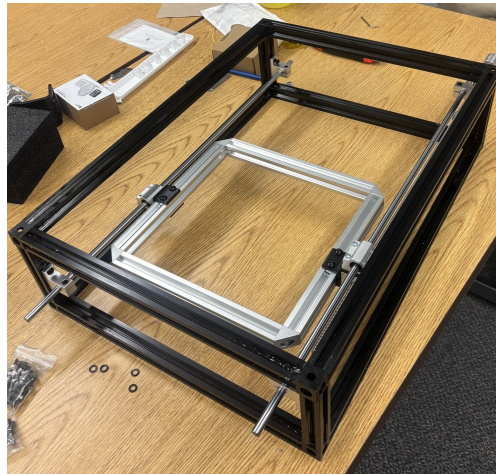
Figure 44: Aluminum Framing Connected through the cube connectors.
