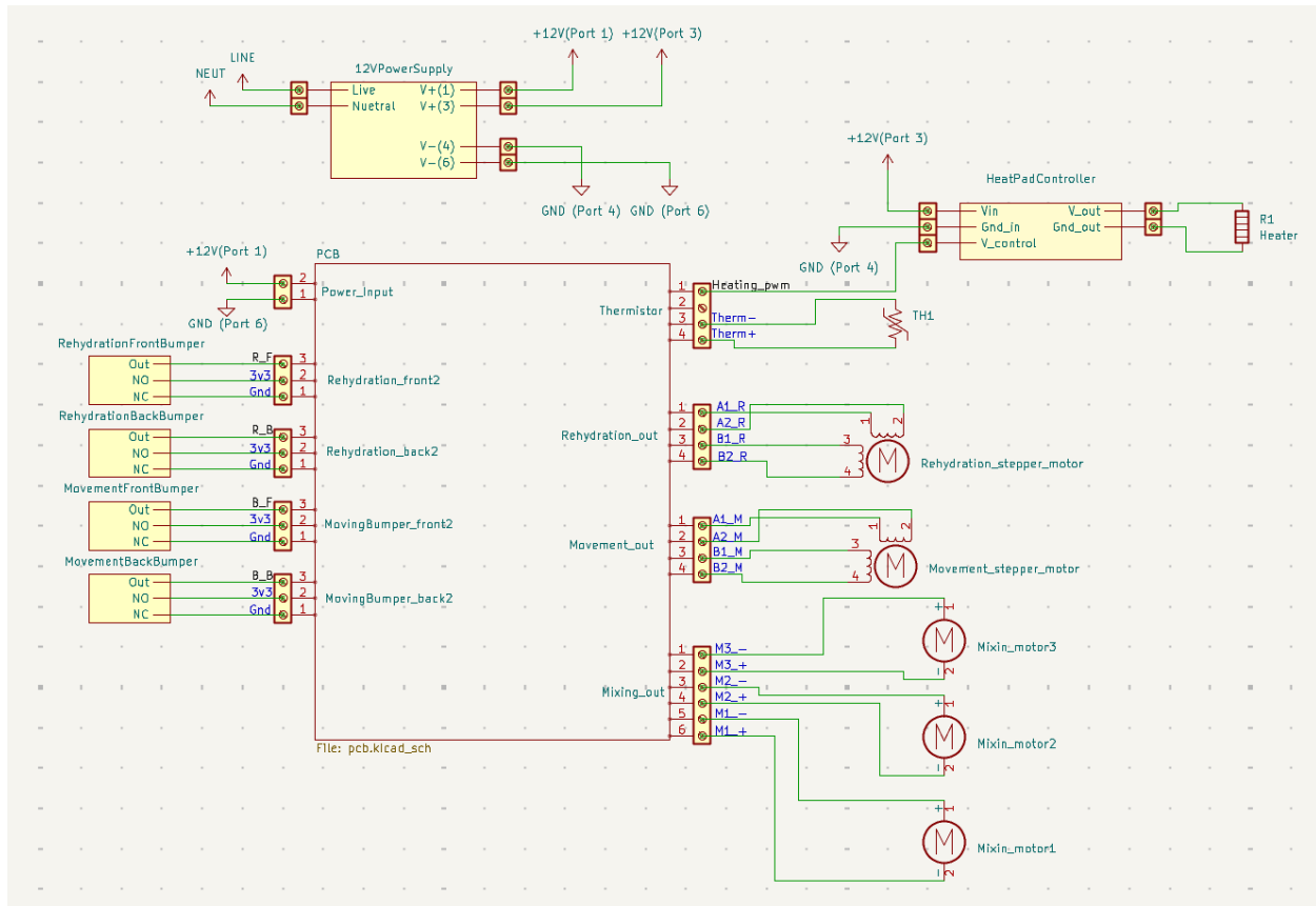
Figure 35: Top level engineering schematic of all electrical components
