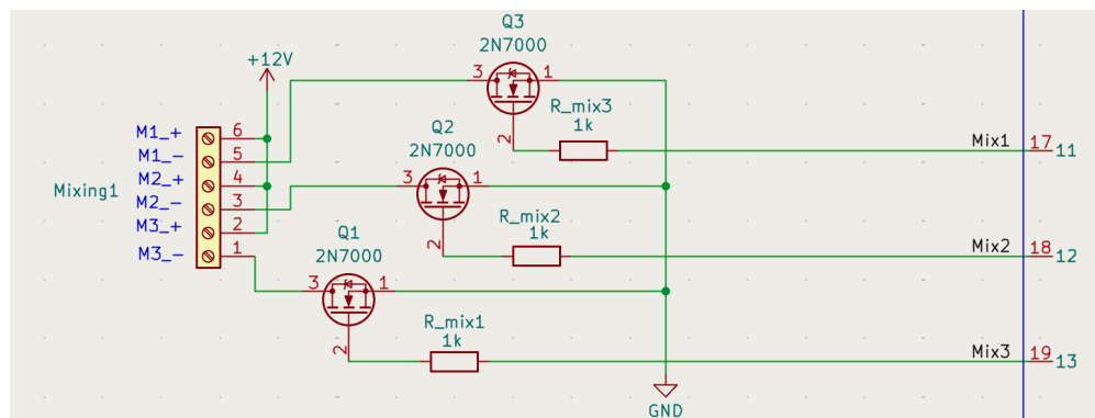
Figure 15: Mixing circuit: three 2N7000 N-channel MOSFETs, each controlled by an ESP32 GPIO pin, regulate power to individual DC mixing motors
