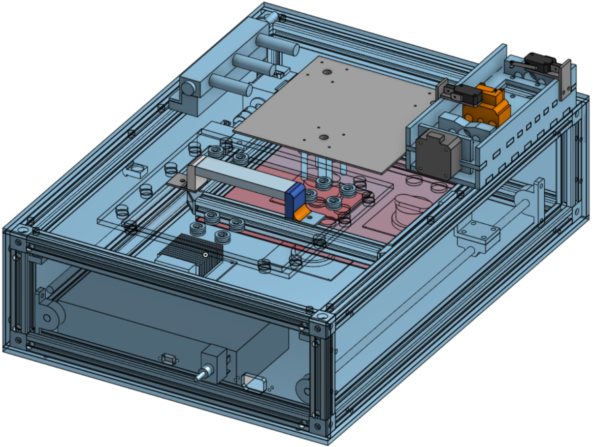
Figure 41: CAD model of wet/dry Cyclor.
