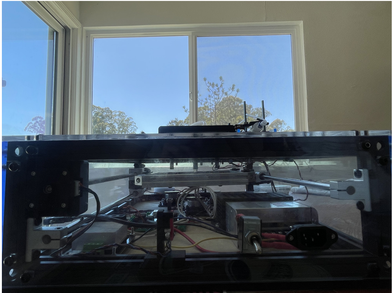
Figure 51: Front profile of the wet/dry Cycler, including power switch and indicator lights.
