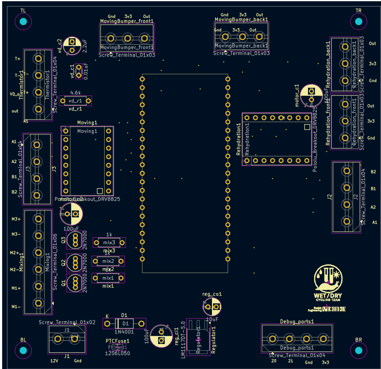
Figure 39: Silkscreen layer of designed PCB
