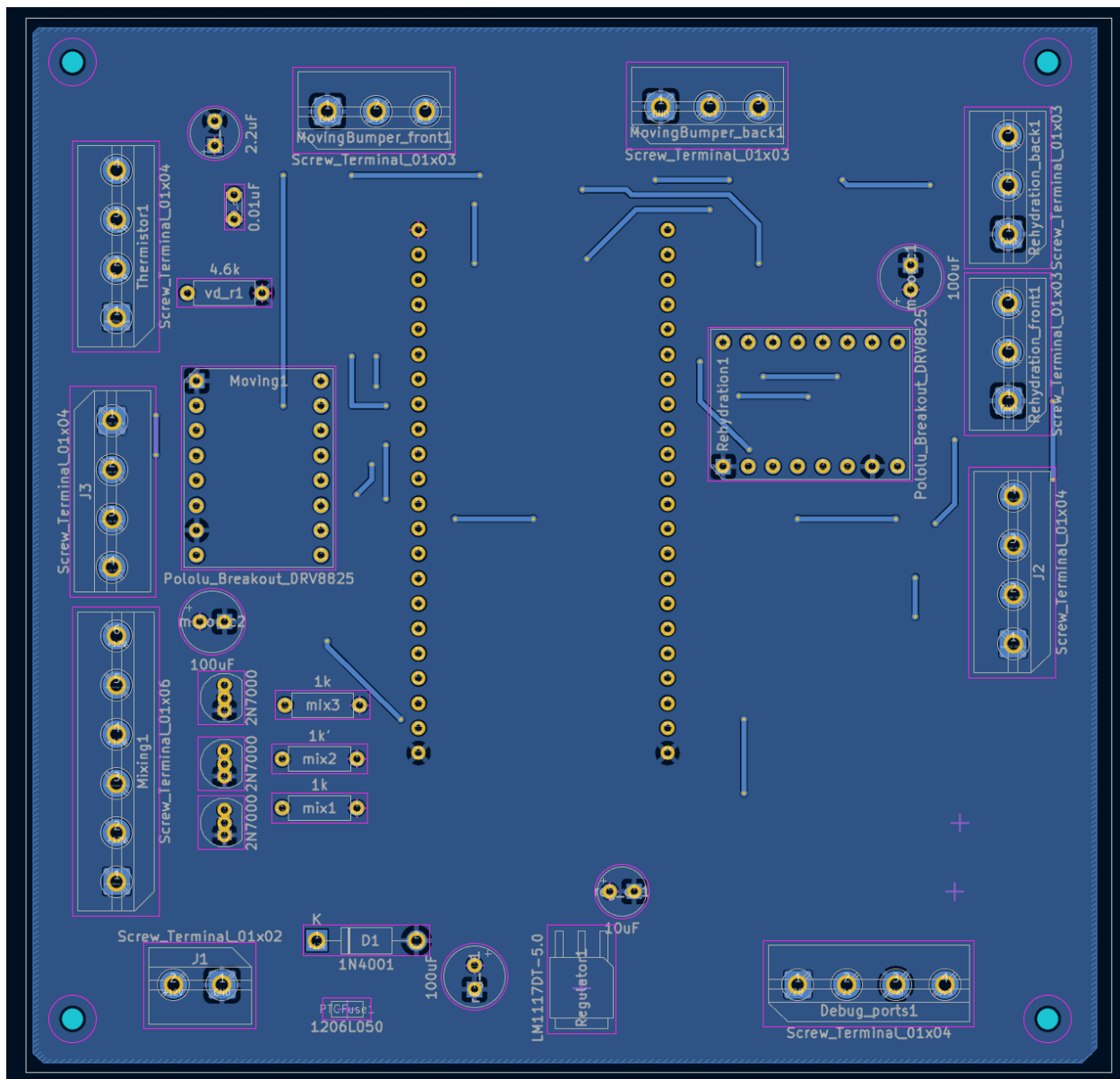
Figure 38: Bottom layer of designed PCB
