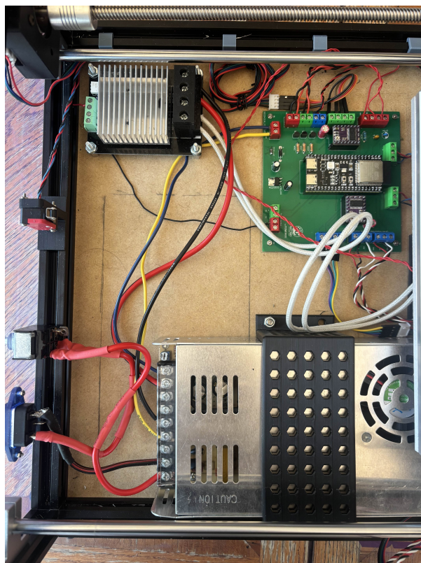
(a) Power supply, MOSFET, and PCB.
