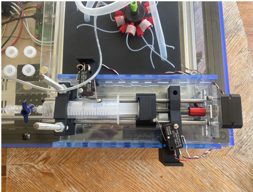
Figure 10: Syringe Pump
