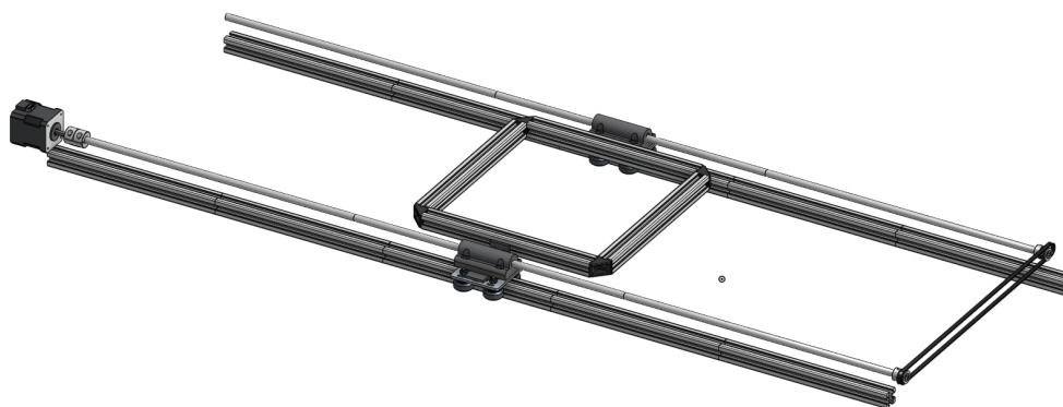
Figure 18: Original prototype extraction mechanism with wheel-mounting platform
