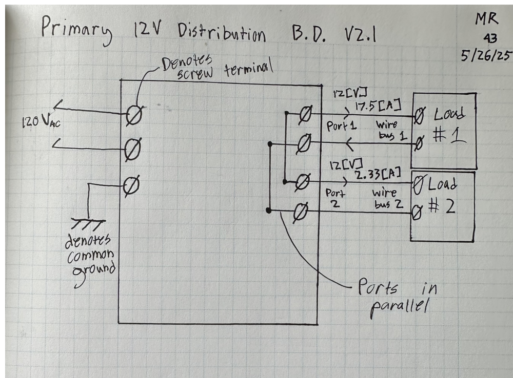
Figure 34: Block diagram of the 12 V power supply and load connections
