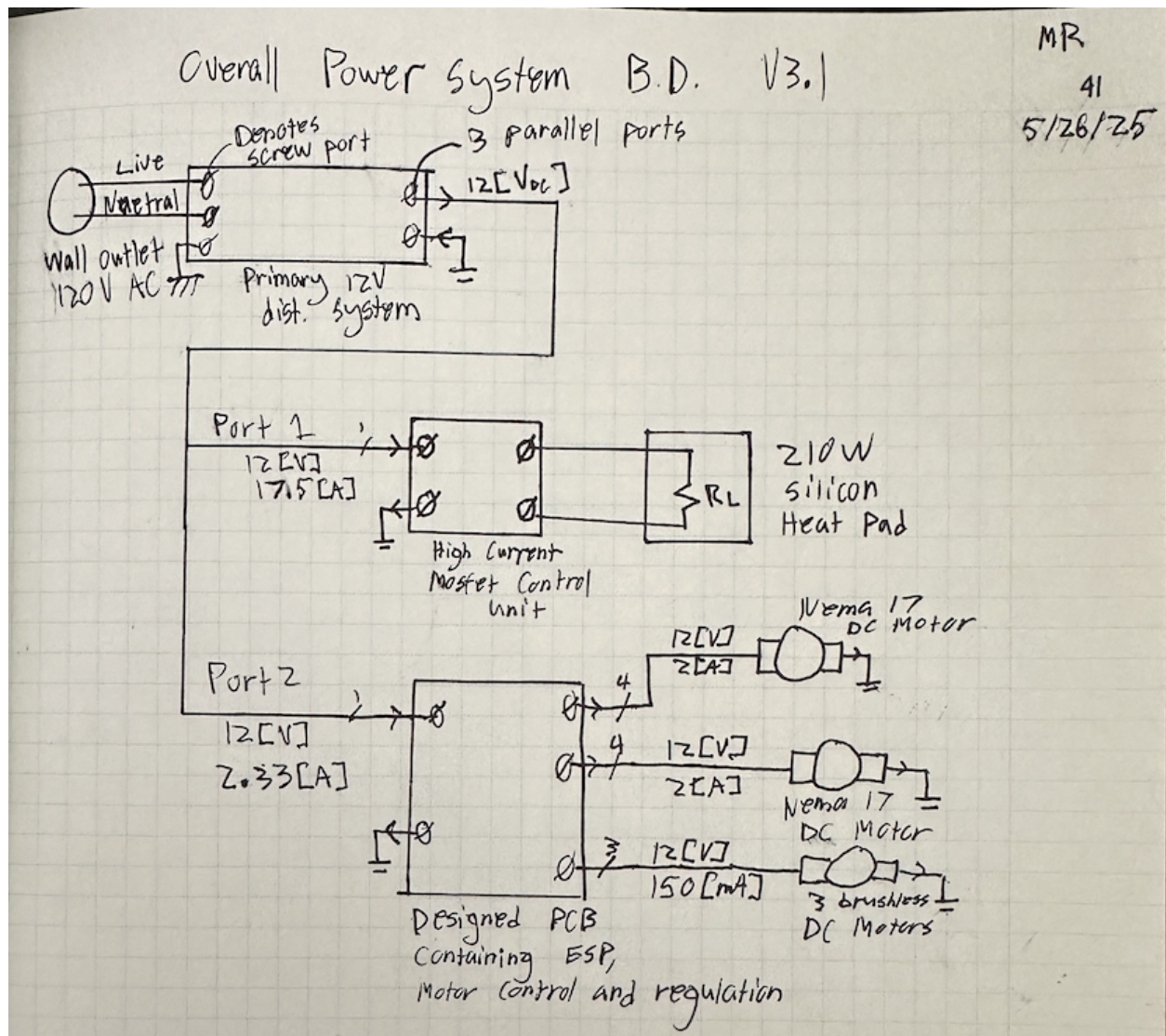
Figure 33: Power system block diagram V3.1
