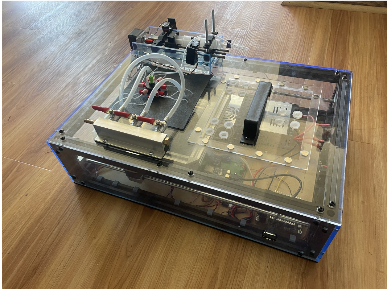
Figure 40: Physical build of the wet/dry Cyclor.
