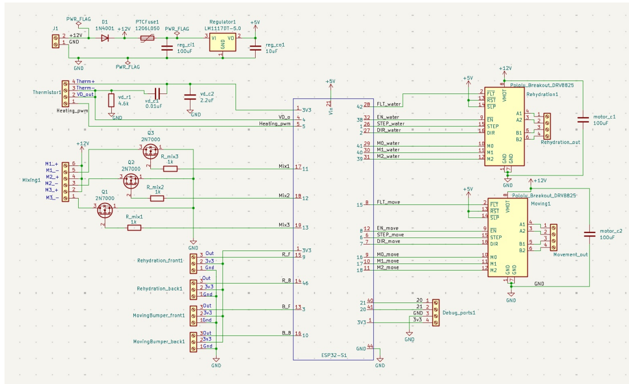
Figure 36: PCB schematic showing relevant components and interconnections
