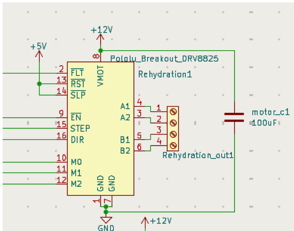
Figure 24: DRV8825 stepper motor driver circuit used for the rehydration syringe pump.
