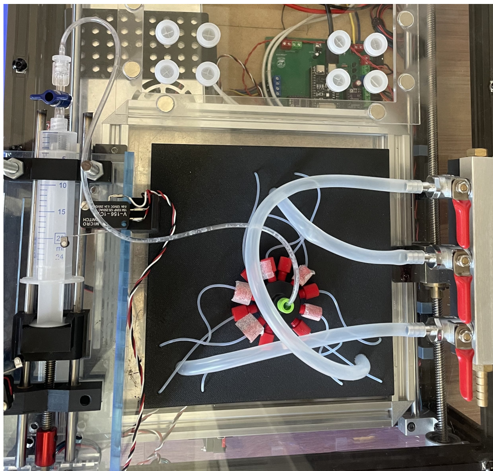
Figure 11: Syringe Pump with Manifold connection
