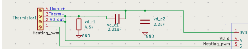
Figure 3: Voltage divider circuit, uses thermistor and known resistor of 4.6KOhm
