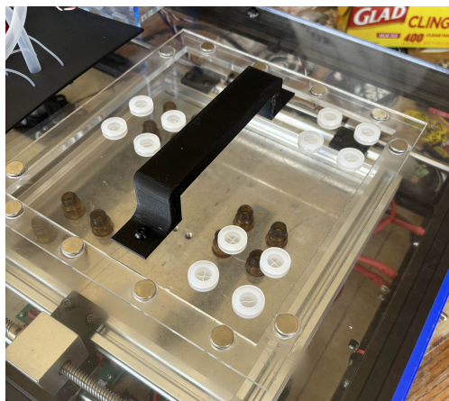
Figure 46: Removable lid system, magnetically attached.
